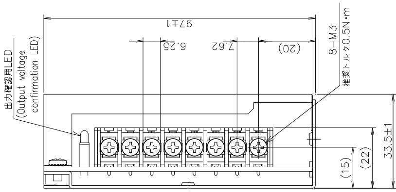
・端子台接続表 Connection of terminal block
