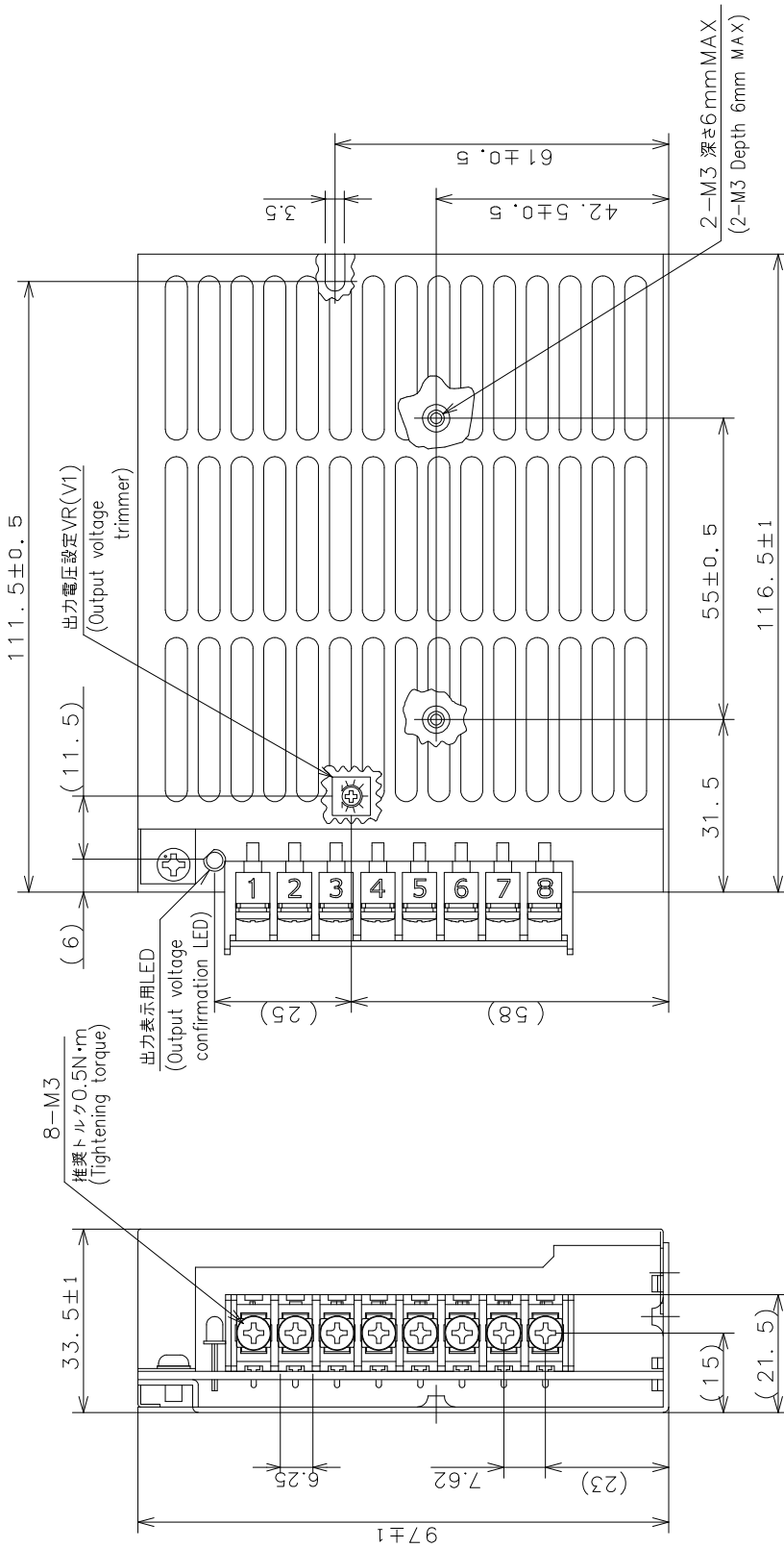
・端子台接続表 Connection of terminal block
