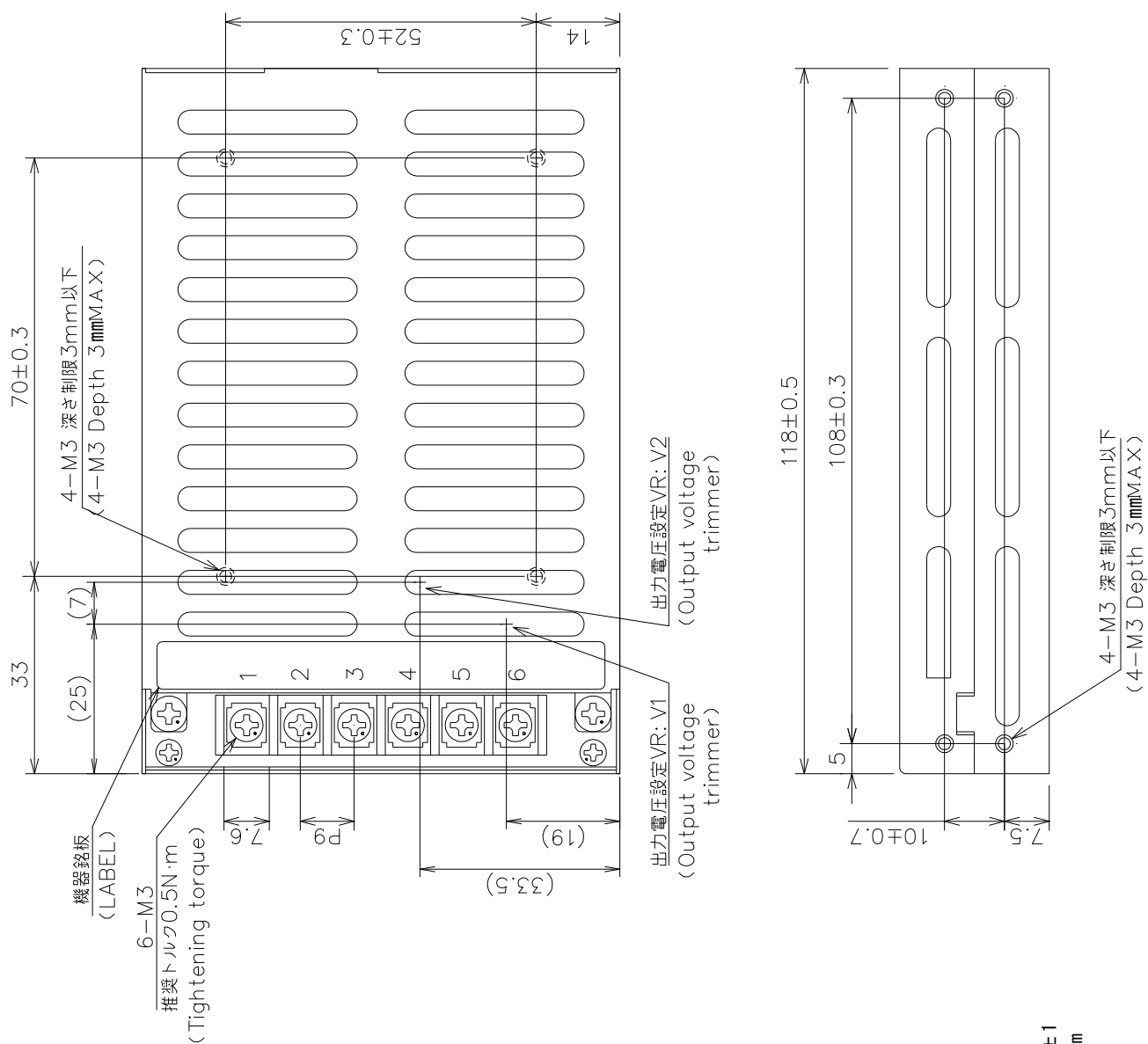
・端子台接続表 Connection of terminal block
